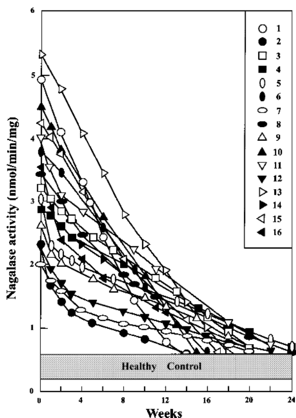
Figure 3. Time course study of GcMAF therapy of 16 prostate cancer patients with serum \alpha -N-acetylgalactosaminidase (Nagalase) as a prognostic index.
