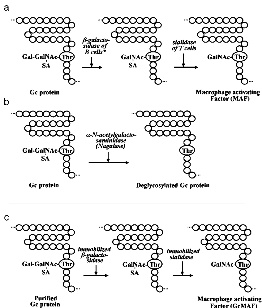
Figure 1. Schematic illustration of the formation of MAF (a), deglycosylation of Gc protein (b), and stepwise treatment of Gc protein with immobilized \beta -galactosidase and sialidase to generate GcMAF (c). Asterisk (*) indicates inflammation-primed B cells: B cells can be treated with an inflamed membranous lipid metabolite, e.g., lysophosphatidylcholine.
