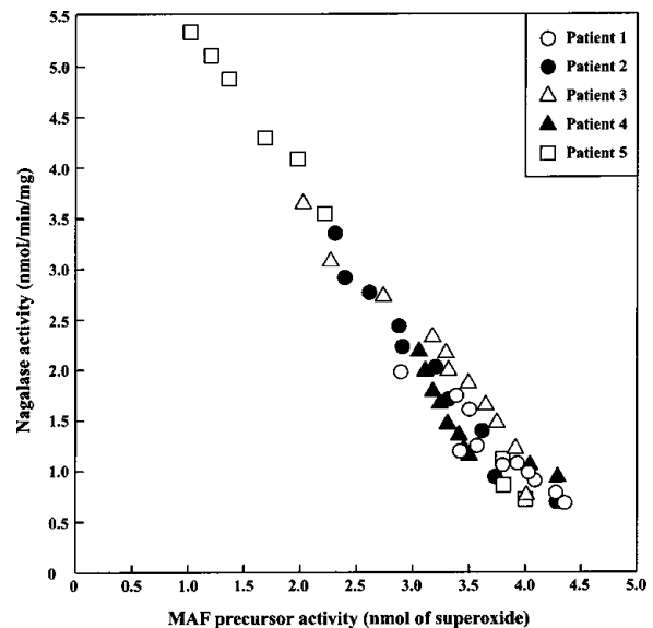
Figure 2. Inverse correlation between the MAF precursor activity of serum Gc protein and serum \alpha -N-acetylgalactosaminidase (Nagalase) activity of prostate cancer patients during GcMAF therapy.
